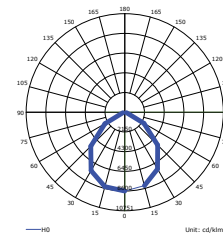
LUMINOUS INTENSITY DISTRIBUTION DIAGRAM
