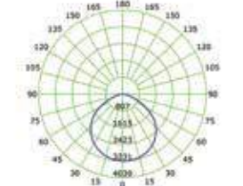
The Average Illuminance Effective Figure
