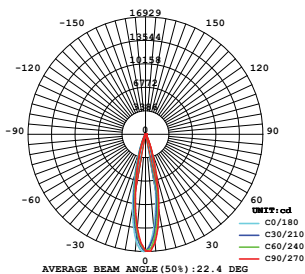
LUMINOUS INTENSITY DISTRIBUTION
