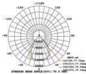
INDOOR INTENSITY DISTRIBUTION DIAGRAM
